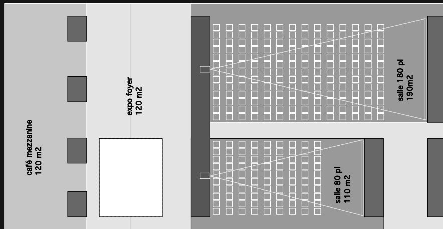
PLAN NIVEAU +1
